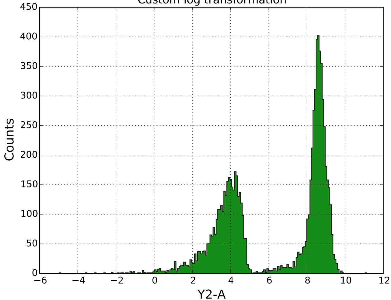
Custom log transformation
