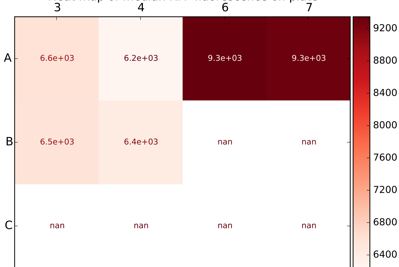
Heat map of median RFP fluorescence on plate
